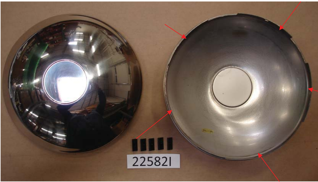
P/N 22582I – has 5 Notches – Arrows are pointing at each notch
